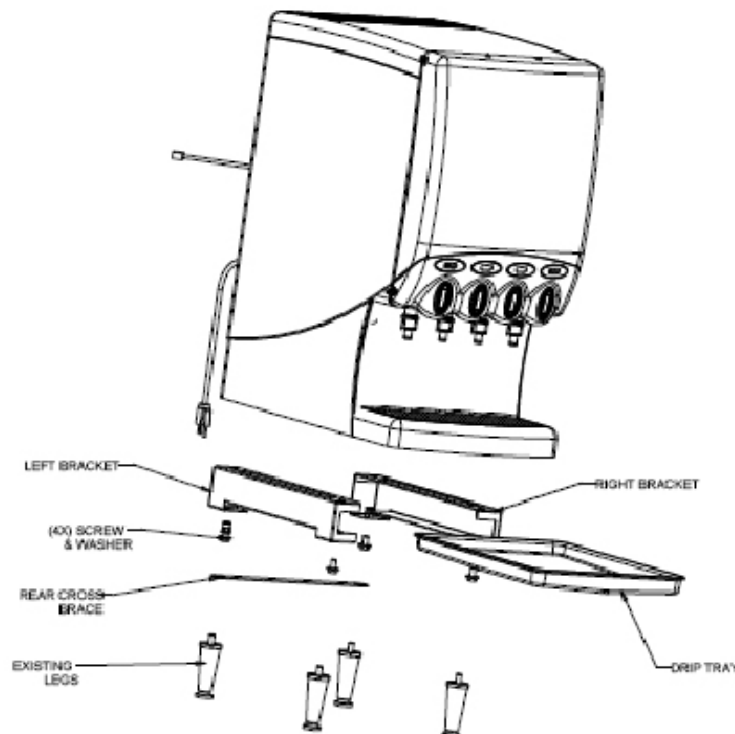
Figure 1. Kit Assembly
